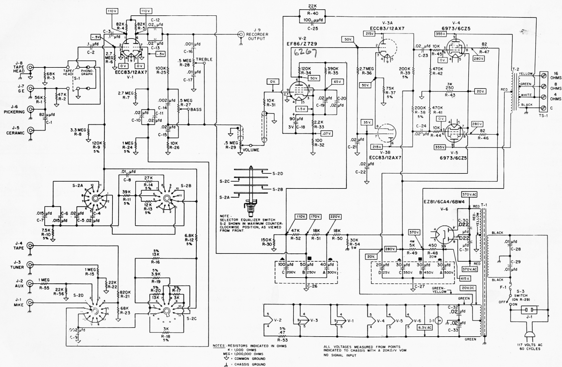
FIGURE 19. SCHEMATIC DIAGRAM
